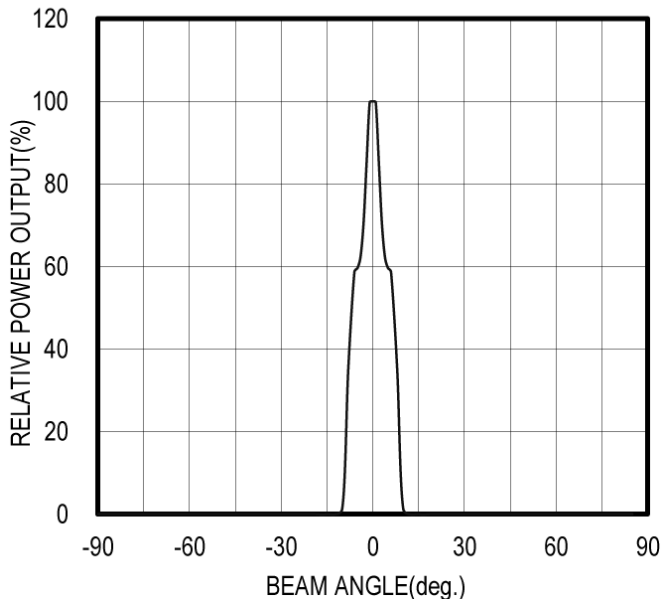
RADIATION PATTERN
