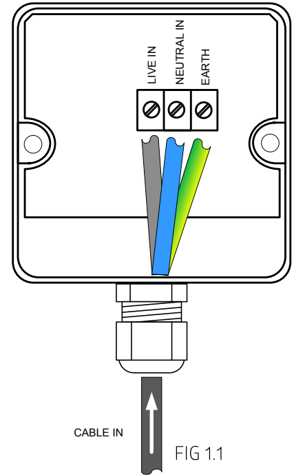
Transmitter - MAINSLINK-TX
